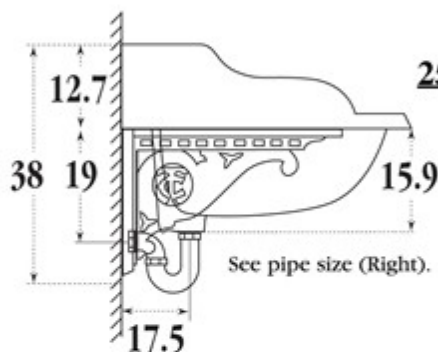
Three-hole 25" Basin.
