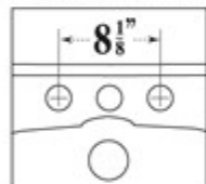
Three-hole 25" Basin.
