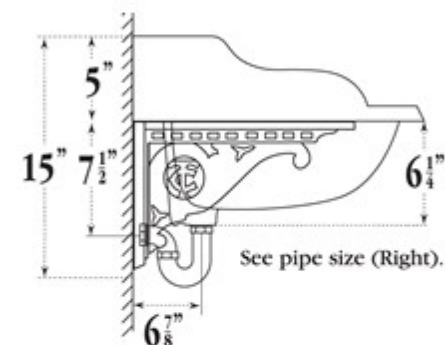
Three-hole 25" Basin.
