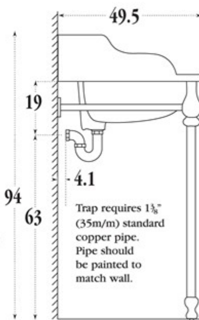
Three-hole 25" Basin.
