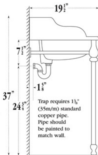
Three-hole 25" Basin.
